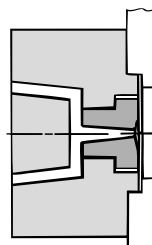
Sprue gate
