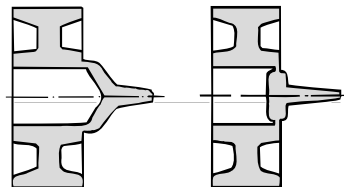
Ring gate
